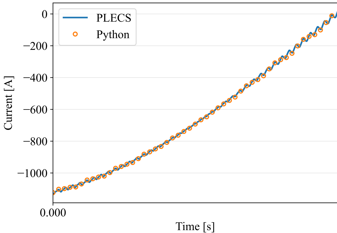
Grid-side current.
